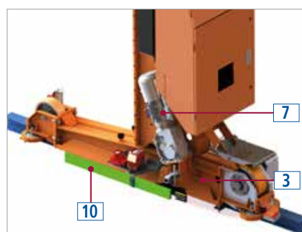
Bottom guide base (3), elevator motor (7) and power supply (10)
