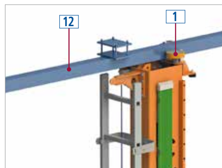
Top guide base (1) and upper track (12)
