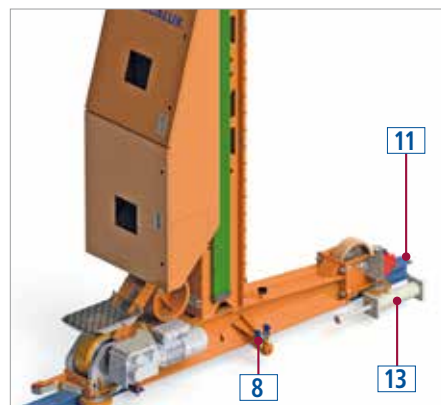
Lower track (11), hydraulic adjustment stop (13) and telemeter (8)
